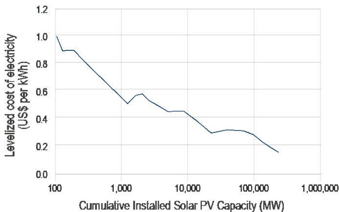
Figure 28: Declining cost of solar PV electricity as installed capacity increases
