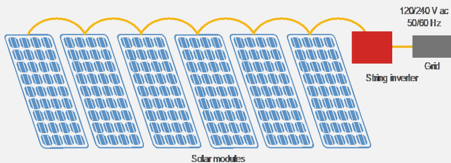
Figure 6: Solar PV system using string inverters
