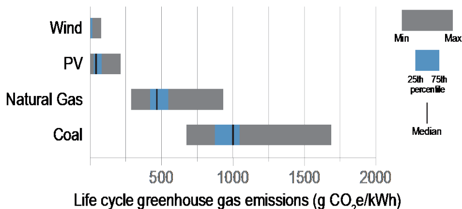
Figure 26: Comparison of life cycle GHG emissions for different types of generators
