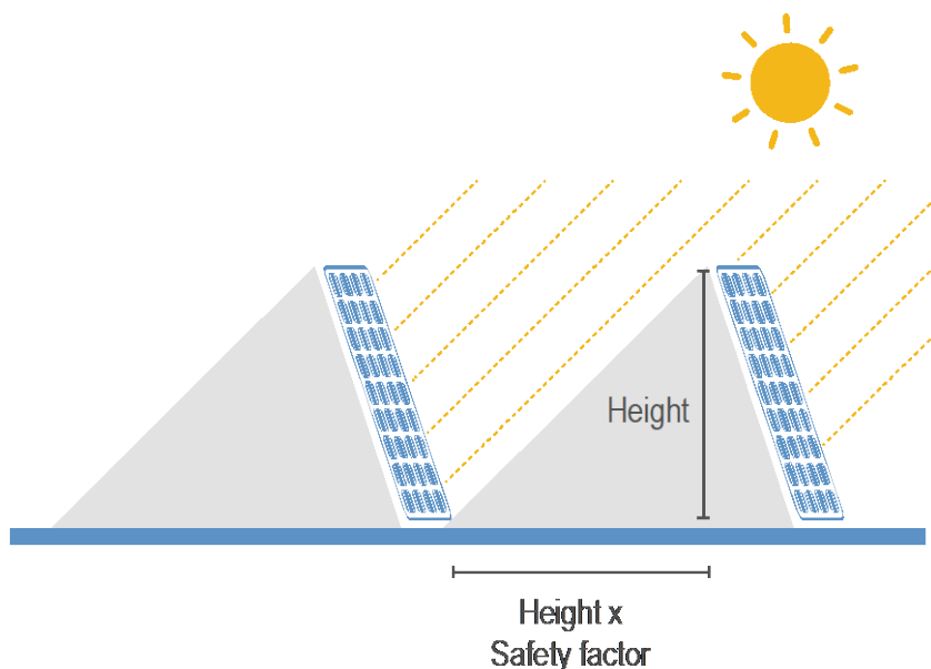
Figure 20: Spacing requirements on flat roofs with tilted racking
