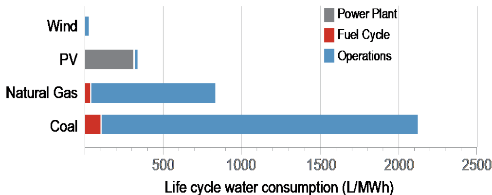
Figure 27: Comparison of life cycle water use for different types of generators
