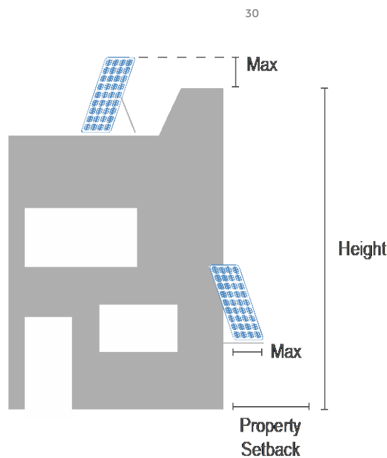
Figure 2: Building height and setback restrictions for solar PV systems
